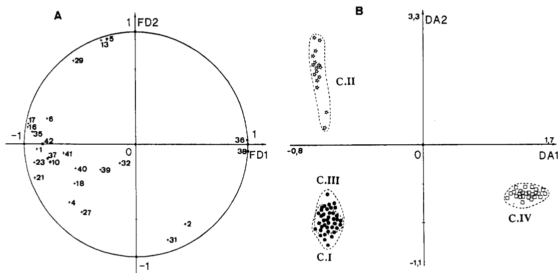
Figure 1. Niaouli essential oil chemotype differentiations using FDA of chemical composition obtained by gas chromatography. (A) Factor loading of variables on the two first discriminant axes. For compound identification see Table 2. (B) Two-dimensional plot of chemotypes I (*), II (☆), III (●), and IV (□) on FDA axes 1 and 2.
